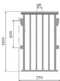
7053077 Handrail 1100/770 12.5 kg
