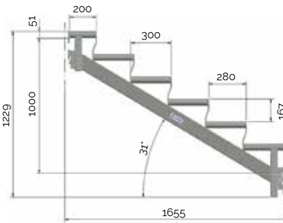
7102100 Stair stringer 1655x1000 24.0 kg
