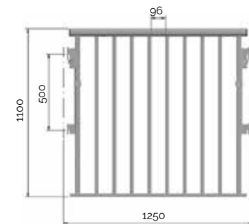
7053125 Handrail 1100/1250 17.5 kg
