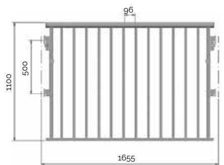
7053165 Handrail 1100/1655 23.0 kg
